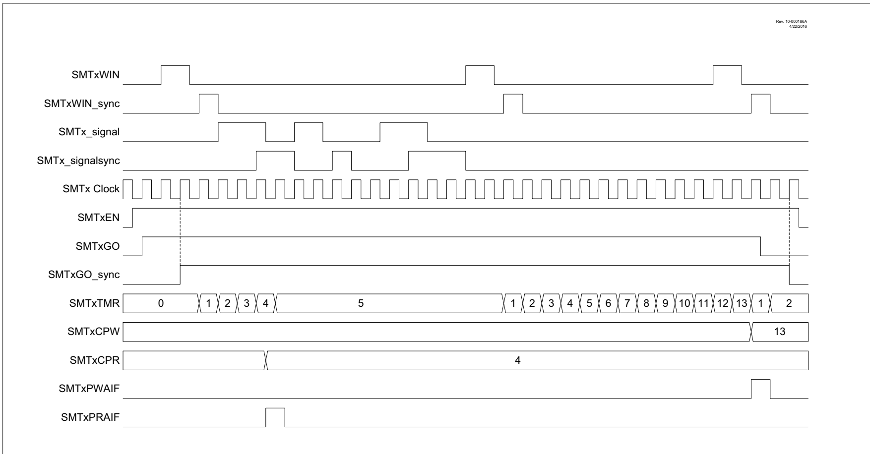
PIC16(L)F19155/56/75/76/85/86
