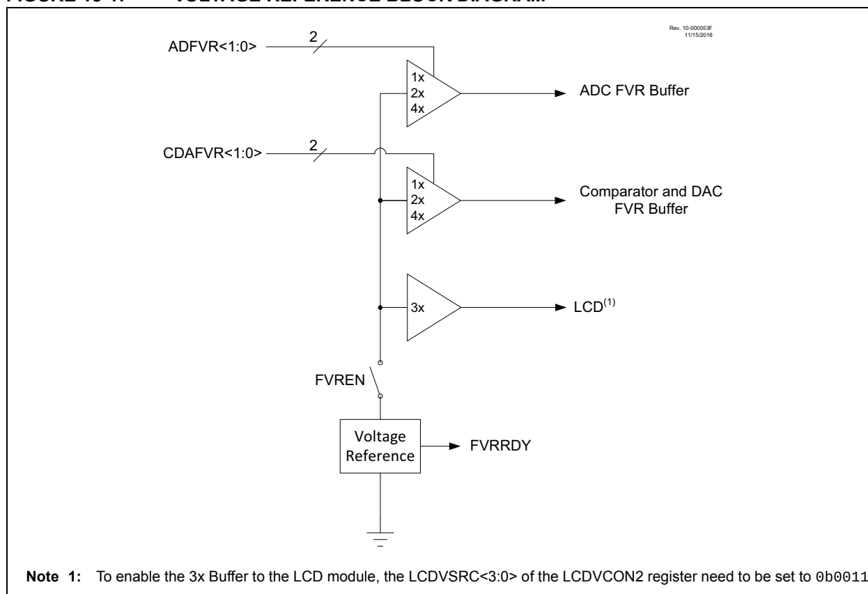
FIGURE 18-1: VOLTAGE REFERENCE BLOCK DIAGRAM
