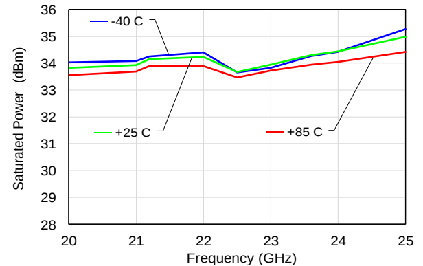
Saturated Power vs. Frequency vs. Temperature
