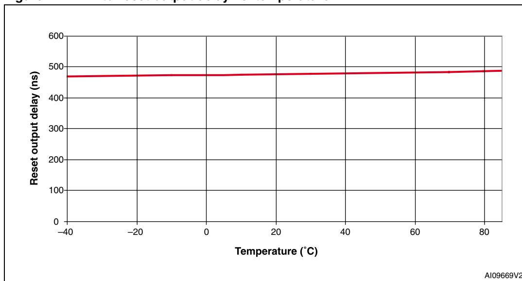
Figure 17. \overline{MR} -to-reset output delay vs. temperature
