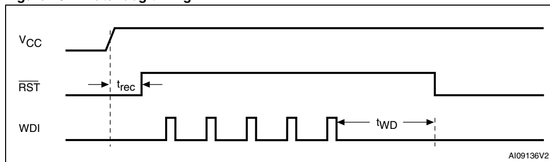
Figure 26. Watchdog timing
