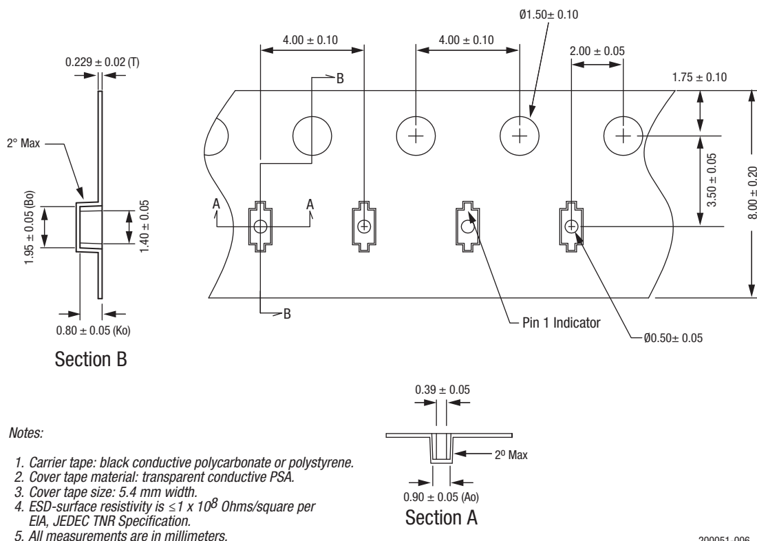
Figure 8. SC-79 Tape and Reel Dimensions
