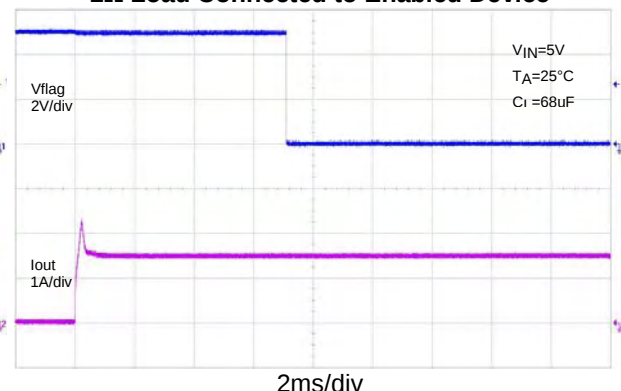
2Ω Load Connected to Enabled Device
