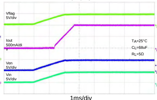
Power On
