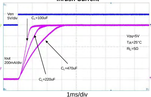
Inrush Current
