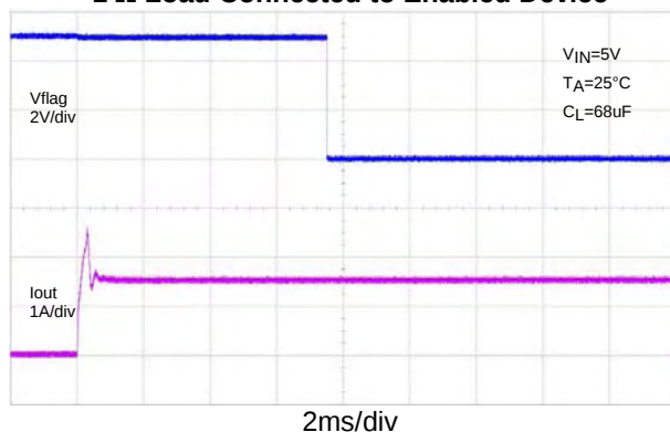
1 Ω Load Connected to Enabled Device
