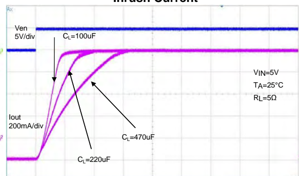
Inrush Current
