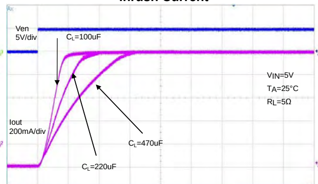
Inrush Current
