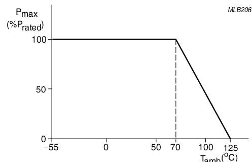
Fig. 6-1 Maximum dissipation ( P_{max} ) in percentage of rated power as a function of the operating ambient temperature ( T_{amb} )
