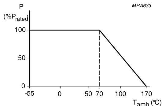
Fig. 6-2 Maximum dissipation ( P_{max} ) in percentage of rated power as a function of the operating ambient temperature ( T_{amb} )
