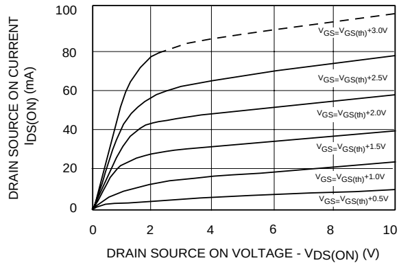
OUTPUT CHARACTERISTICS
