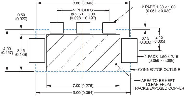
3 Way Right Angle Battery Connector PCB Layout
