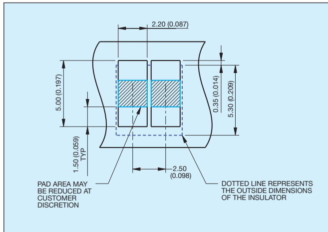
2 Way Reduced Battery Connector PCB Layout
