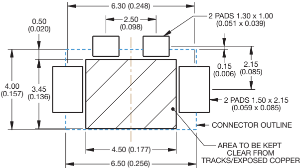
2 Way Right Angle Battery Connector PCB Layout
