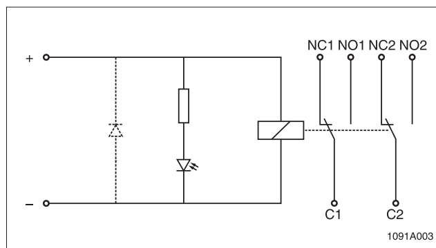
Figure 3. UMK 22-RELAY Block Diagram
