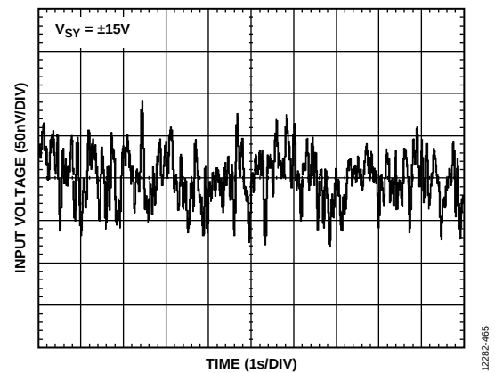
Figure 73. 0.1 Hz to 10 Hz Noise, V_{SV} = \pm 15\text{ V}
