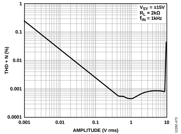
Figure 72. THD + N vs. Amplitude, V_{SV} = \pm 15\text{ V}
