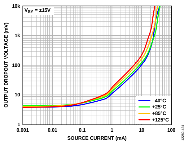
Figure 38. Output Dropout Voltage vs. Source Current, V_{SY} = \pm 15 V
