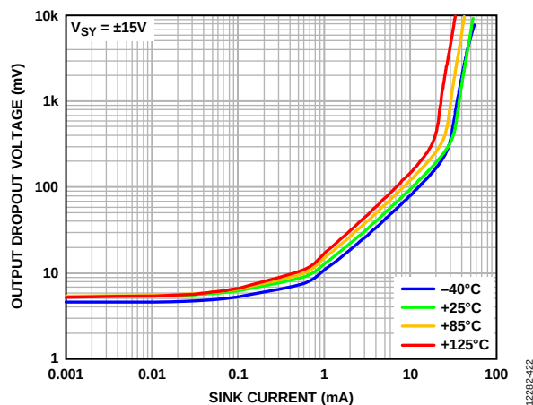
Figure 37. Output Dropout Voltage vs. Sink Current, V_{SY} = \pm 15 V
