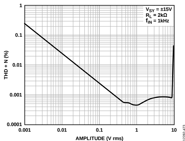
Figure 72. THD + N vs. Amplitude, V_{SY} = \pm 15\text{ V}
