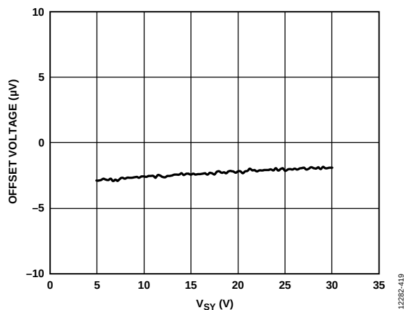
Figure 36. Offset Voltage ( V_{OS} ) vs. Power Supply Voltage ( V_{SY} )
