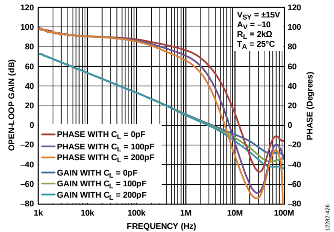
Figure 42. Open-Loop Gain and Phase vs. Frequency, V_{SY} = \pm 15 V
