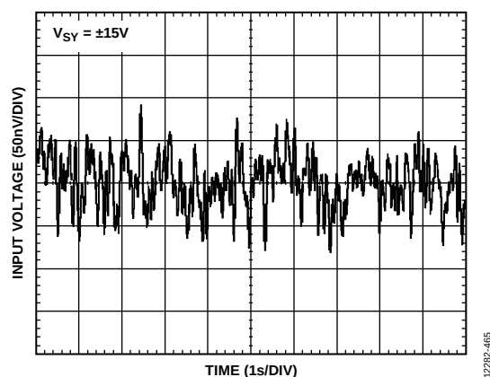
Figure 73. 0.1 Hz to 10 Hz Noise, V_{SY} = \pm 15\text{ V}
