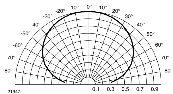
Fig. 11 - Directivity
