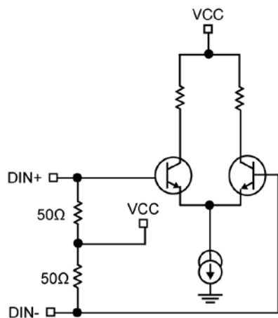
Figure 1a. Simplified Input Stage
