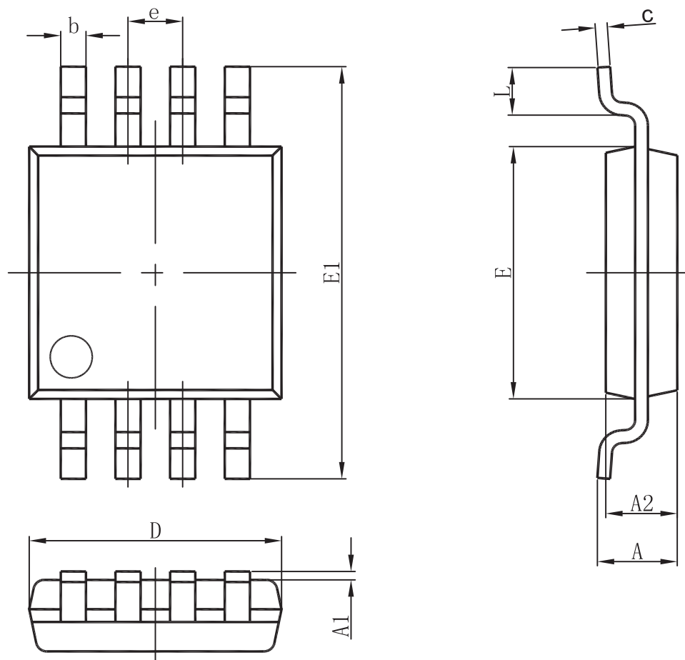
MSOP-8
