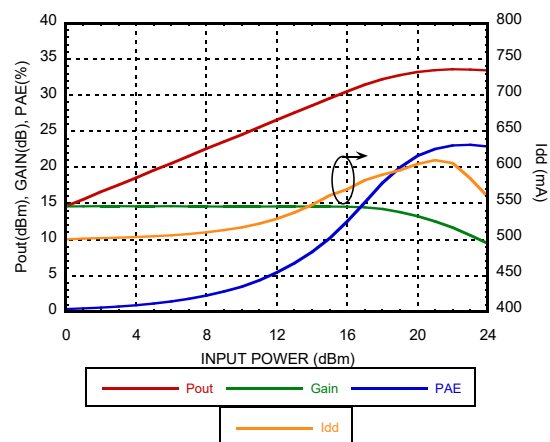
Power Compression @ 10 GHz
