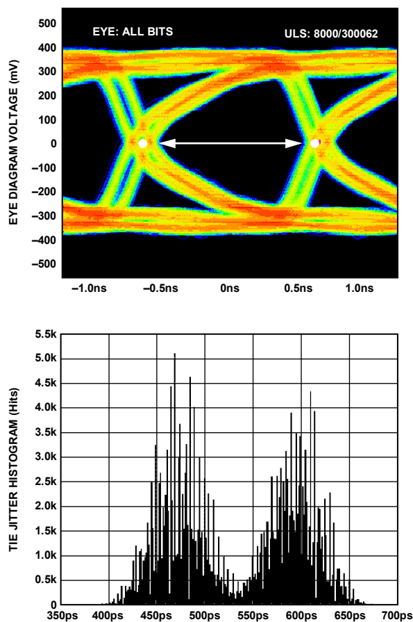
Figure 71. Data Eye for LVDS Outputs in ANSI-644 Mode with Trace Lengths Less than 24 Inches on Standard FR-4 Material, External 100 \Omega Far-End Termination Only
