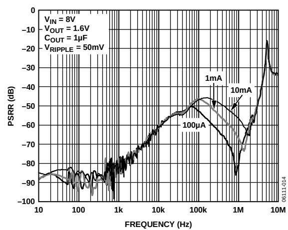
Figure 14. Power Supply Rejection Ratio vs. Frequency (1.6 V Adjustable Output)
