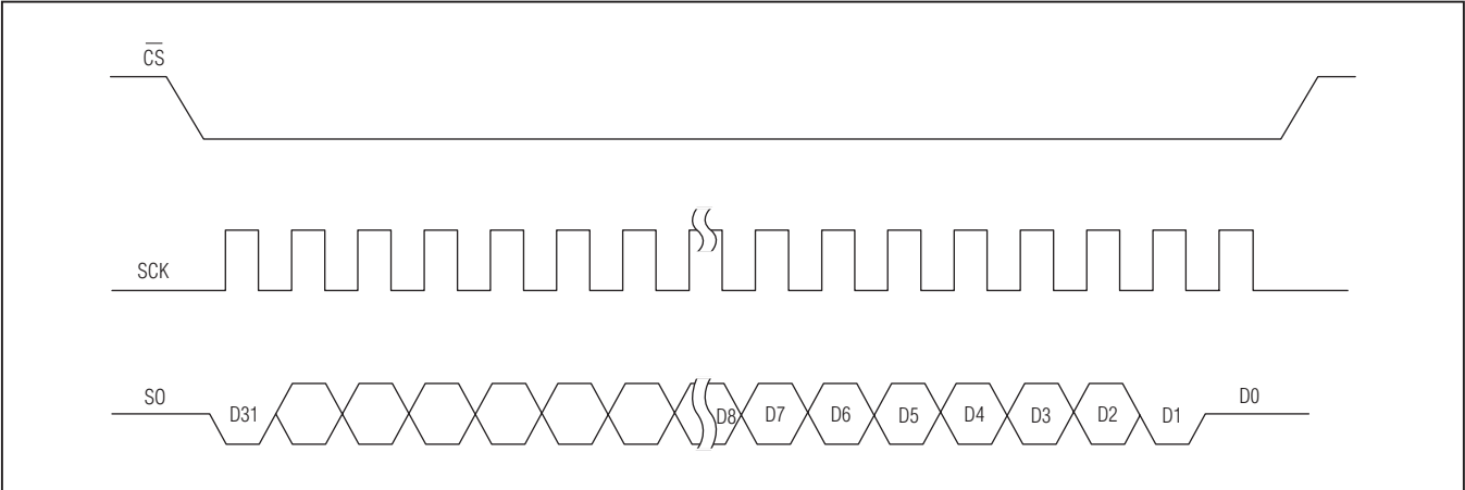
Figure 1. Serial-Interface Protocol
