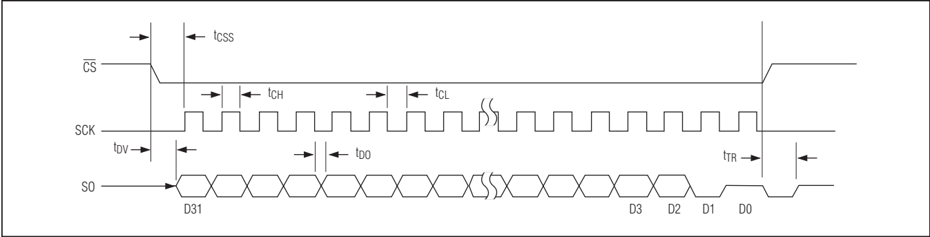
Figure 2. Serial-Interface Timing
