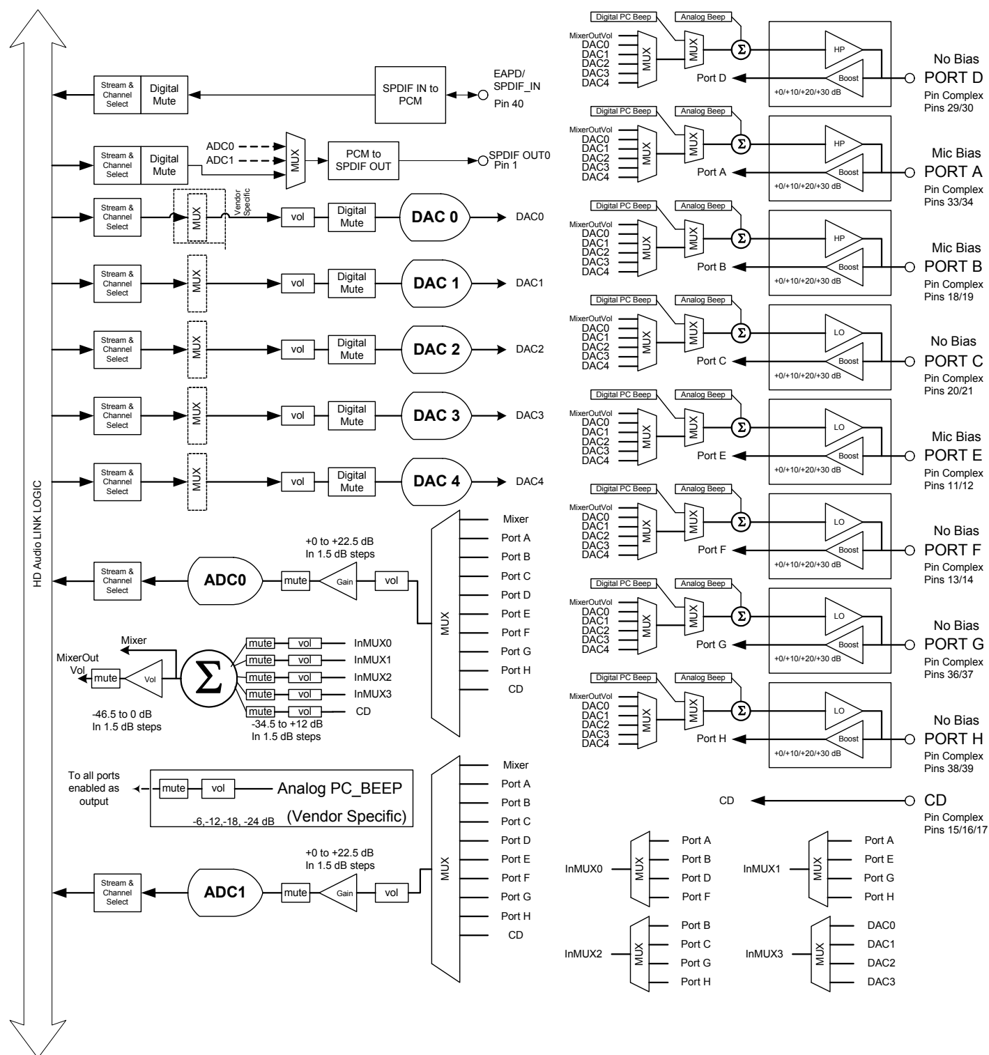
Figure 10. 40QFN Functional Block Diagram
