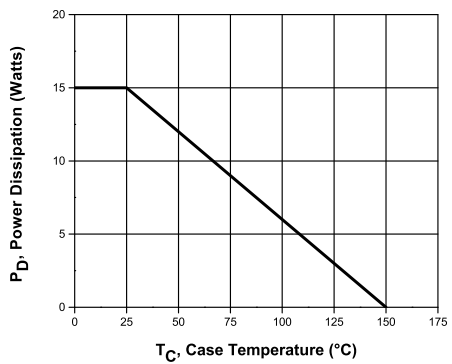
Power Derating
