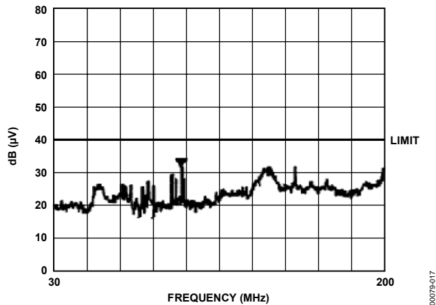
Figure 22. Radiated Emissions
