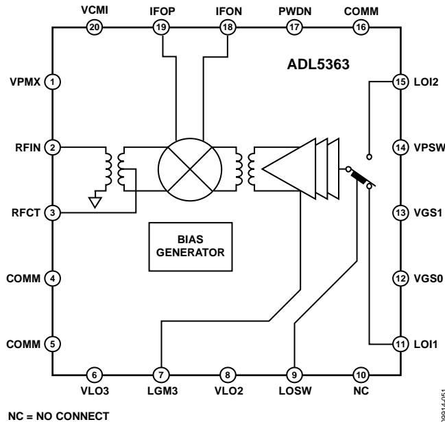
Figure 46. Simplified Schematic
