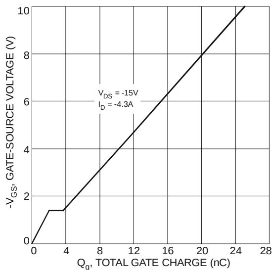
Figure 11 Gate-Charge Characteristics
