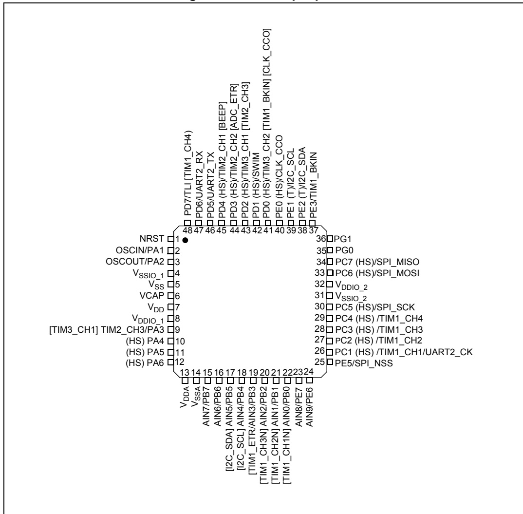
Figure 3. LQFP 48-pin pinout
