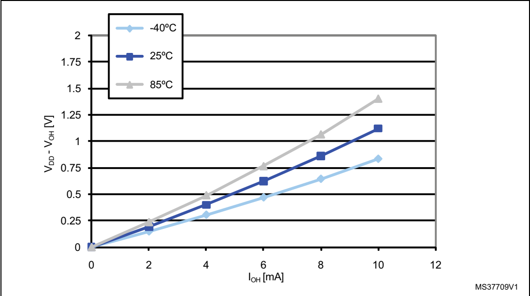
Figure 30. Typ. V_{DD} - V_{OH} @ V_{DD} = 5 V (standard ports)
