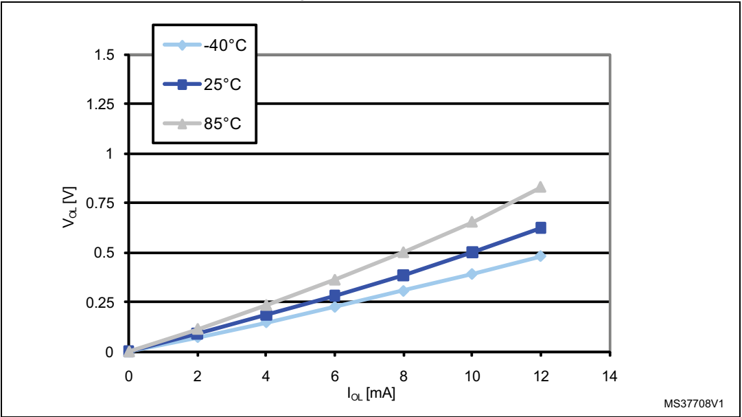
Figure 29. Typ. V_{OL} @ V_{DD} = 3.3 V (high sink ports)
