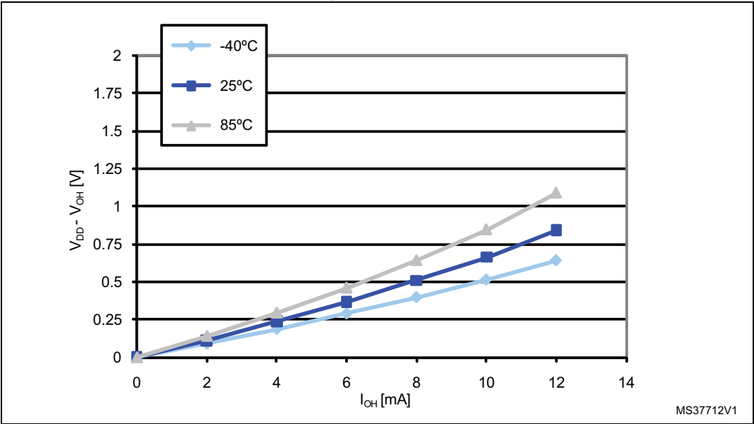
Figure 33. Typ. V_{DD} - V_{OH} @ V_{DD} = 3.3\text{ V} (high sink ports)
