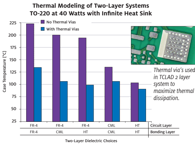
The graph depicts the modeled thermal result of various two-layer constructions as a function of device case temperature. The emphasis is the thermal effect of proper vias utilization.
