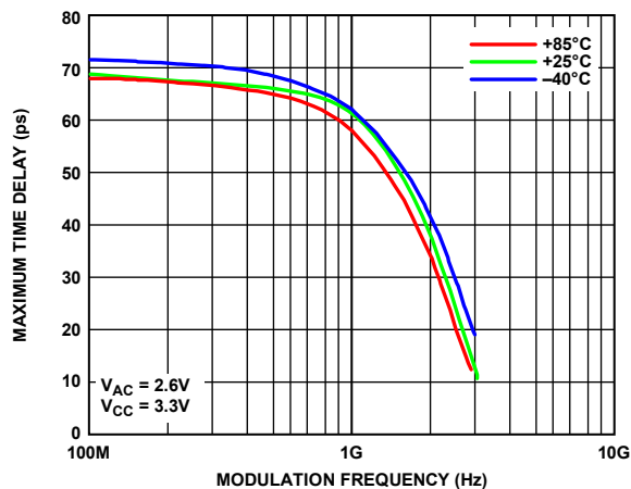
Figure 31. Maximum Time Delay vs. Modulation Frequency, Input Data Rate = 22.5 Gbps, PRBS 2^{23} - 1 , 6 dBm Input Power Applied to V_{DCP} and V_{DCN} Terminated to 50 \Omega
