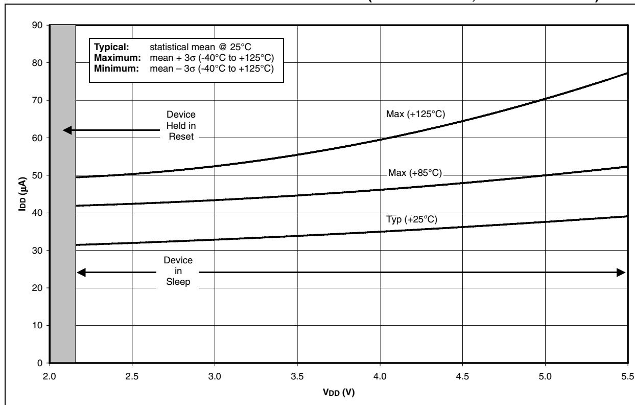
FIGURE 28-16: \Delta I_{BOR} vs. V_{DD} OVER TEMPERATURE (BOR ENABLED, V_{BOR} = 2.00\text{--}2.16\text{V} )
