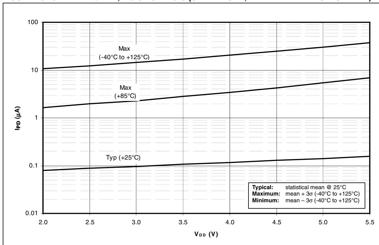
FIGURE 28-15: I_{PD} vs. V_{DD} , -40^{\circ}\text{C} TO +125^{\circ}\text{C} (SLEEP MODE, ALL PERIPHERALS DISABLED)
