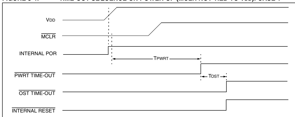
FIGURE 3-4: TIME-OUT SEQUENCE ON POWER-UP ( \overline{\text{MCLR}} NOT TIED TO V_{DD} ): CASE 1
