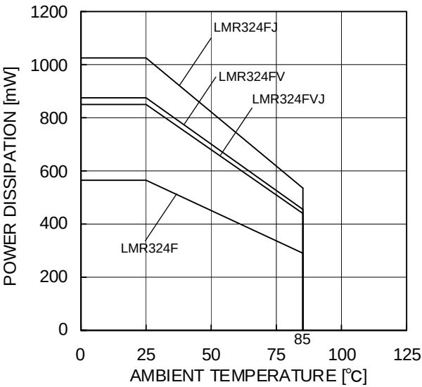
Figure 50. Derating curve
