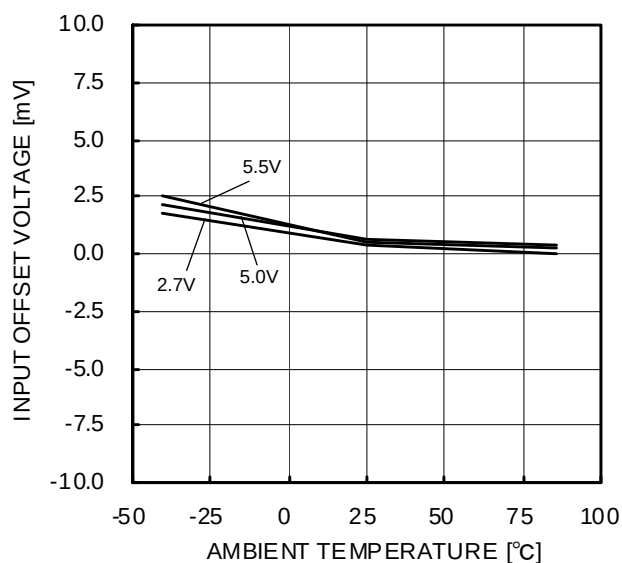
Figure 14. Input Offset Voltage – Ambient Temperature ( V_{in} = V_{DD} , OUT = 0.1V )
