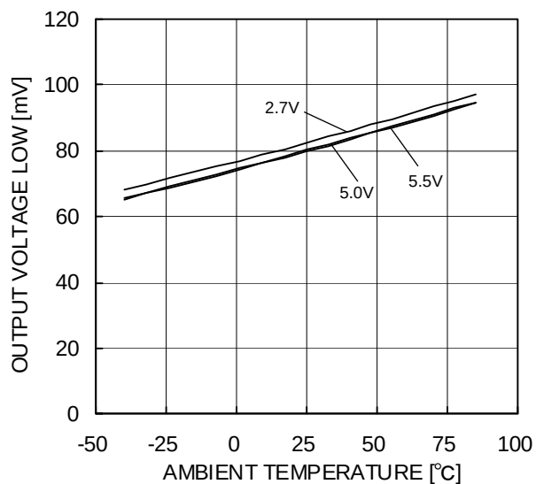
Figure 32. Maximum Output Voltage(Low) – Ambient Temperature ( R_L=2k\Omega )
