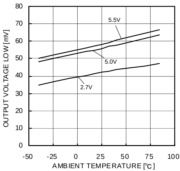
Figure 8. Maximum Output Voltage(Low) – Ambient Temperature ( R_L=2k\Omega )
