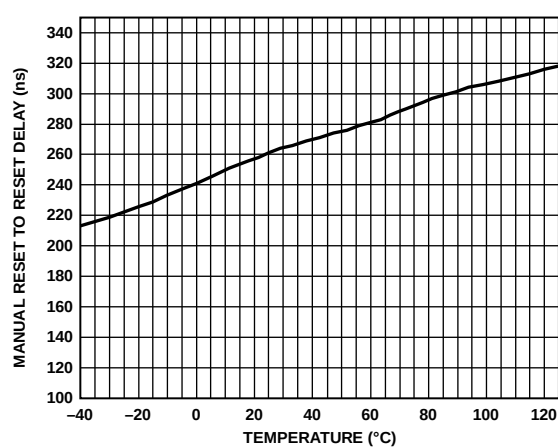
Figure 9. Manual Reset to Reset Propagation Delay vs. Temperature (ADM823/ADM825)
