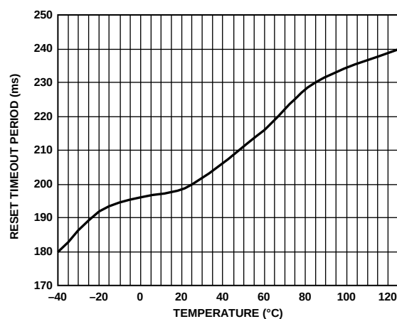
Figure 10. Reset Timeout Period vs. Temperature
