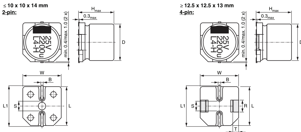
Fig.2 Dimensional outline
