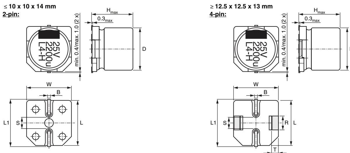
Fig.2 Dimensional outline
