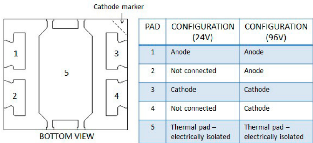
Figure 7. Pad design details for LUXEON 5258.
