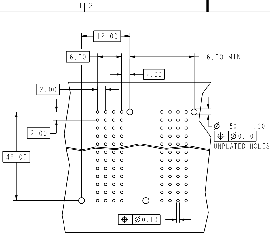
REQUIRED PC BOARD LAYOUT COMPONENT SIDE SEE PRINT 58351 FOR ADDITIONAL PCB INFORMATION
