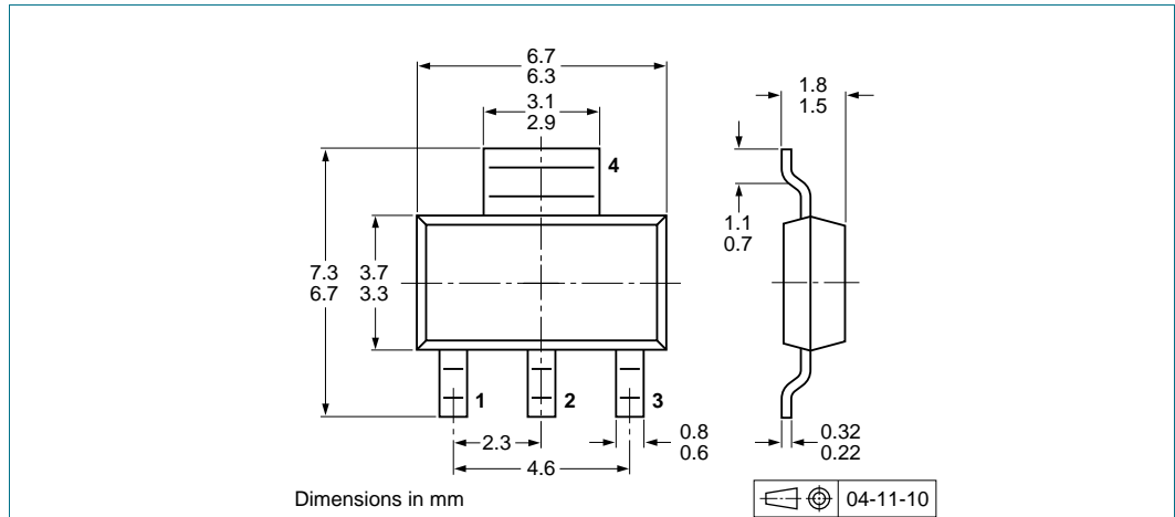
Fig 19. Package outline SOT223 (SC-73)
