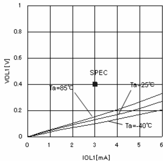
Figure 5. L input voltage V_{OL1-IOL1} ( V_{CC}=2.5\text{V} )
