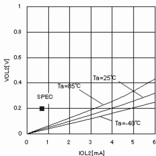
Figure 4. L output voltage V_{OL2-IOL2} ( V_{CC}=1.7\text{V} )
