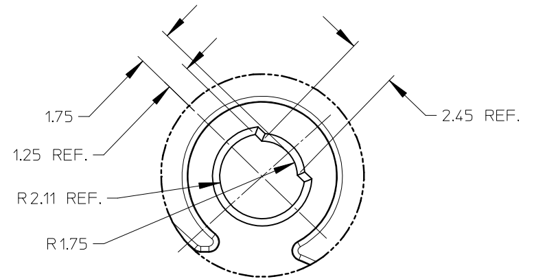
DETAIL 2 SCALE 6:1
