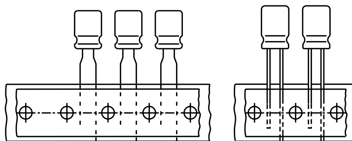
Formed leads for \varnothing D = 8 mm with pitch F = 5 mm
