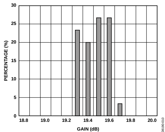
Figure 10. Gain Distribution at 2000 MHz
