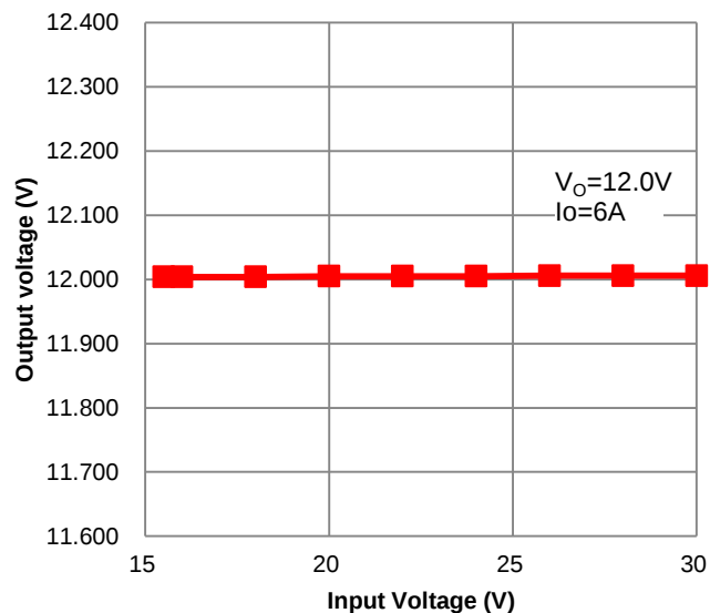
Figure 10. Line regulation
