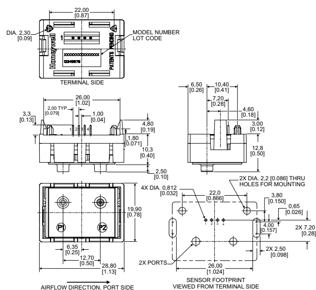
Figure 8. Mounting Dimensions (For reference only: mm [in]). Additional port and housing styles available.
