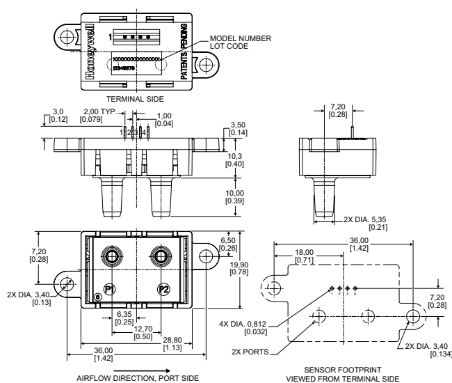
Figure 8. Mounting Dimensions (For reference only: mm [in]). Additional port and housing styles available.
