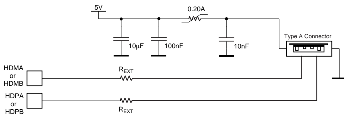
Figure 40-4. Board Schematic to Interface UHP Device Controller
