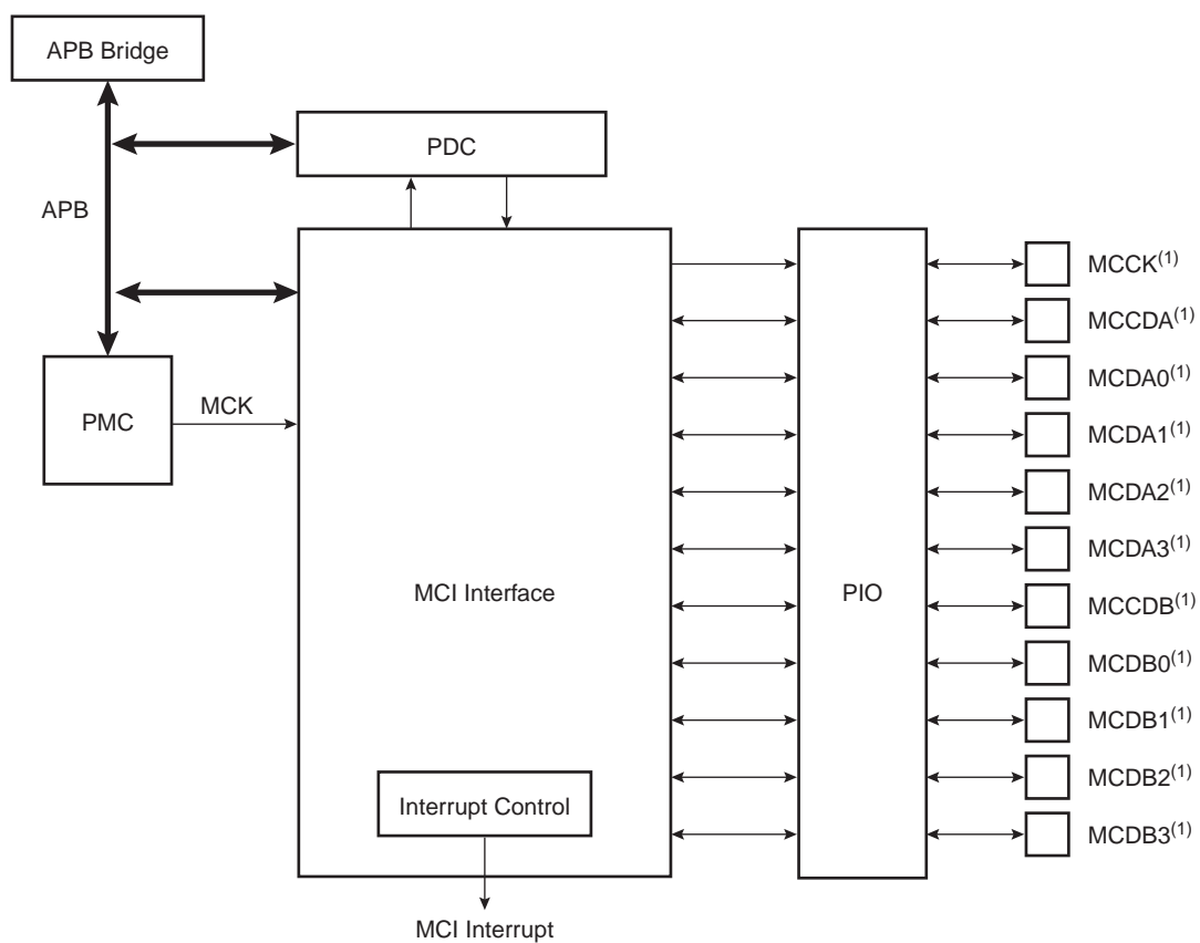
Figure 37-1. Block Diagram
