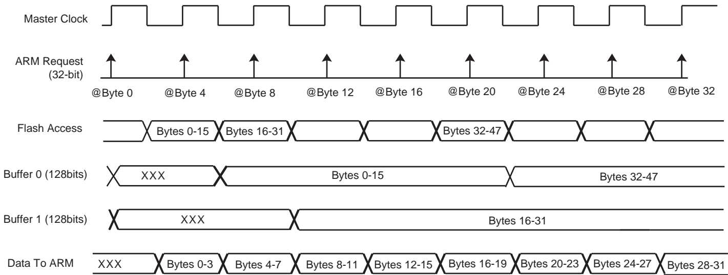
Figure 20-2. Code Read Optimization in ARM Mode for FWS = 0
