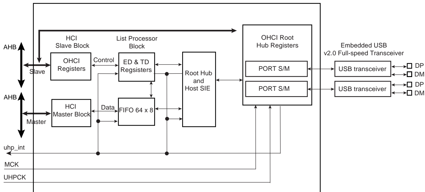
Figure 40-1. Block Diagram
