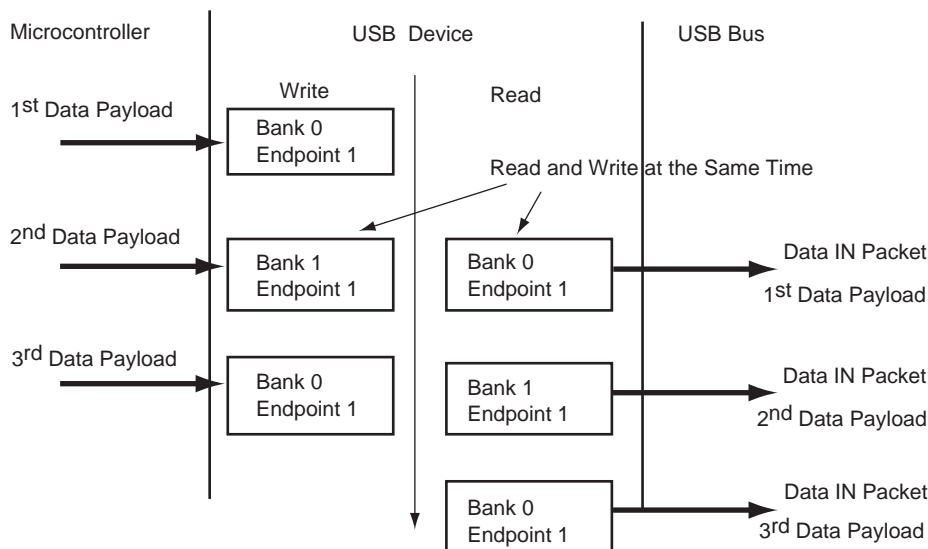
Figure 39-7. Bank Swapping Data IN Transfer for Ping-pong Endpoints
