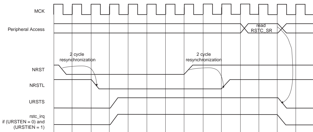
Figure 15-10. Reset Controller Status and Interrupt
