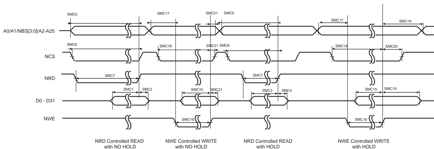
Figure 43-3. SMC Timings - NRD Controlled Read and NWE Controlled Write
