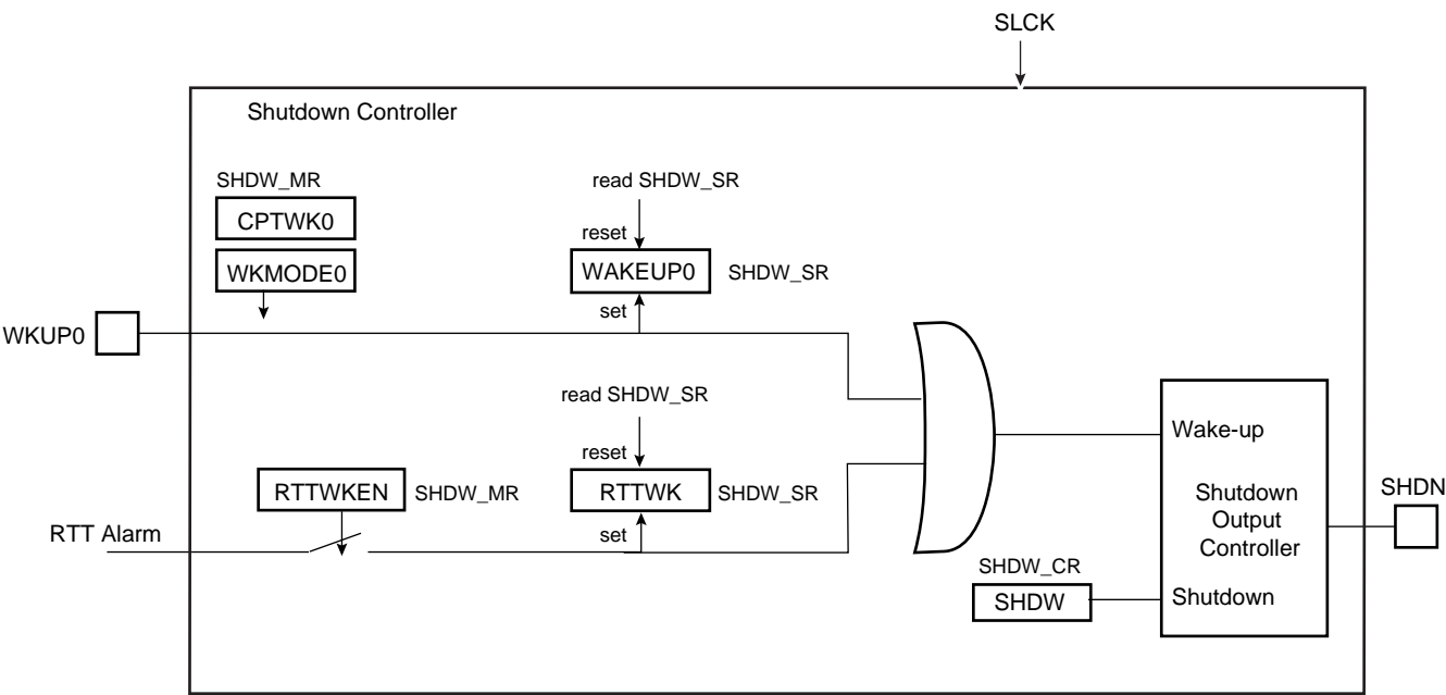
Figure 19-1. Shutdown Controller Block Diagram
