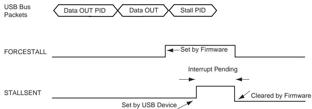
Figure 39-13. Stall Handshake (Data OUT Transfer)
