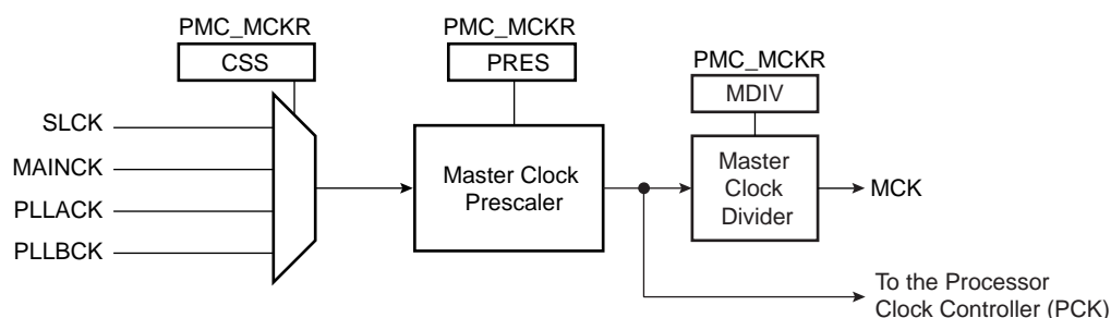
Figure 28-2. Master Clock Controller
