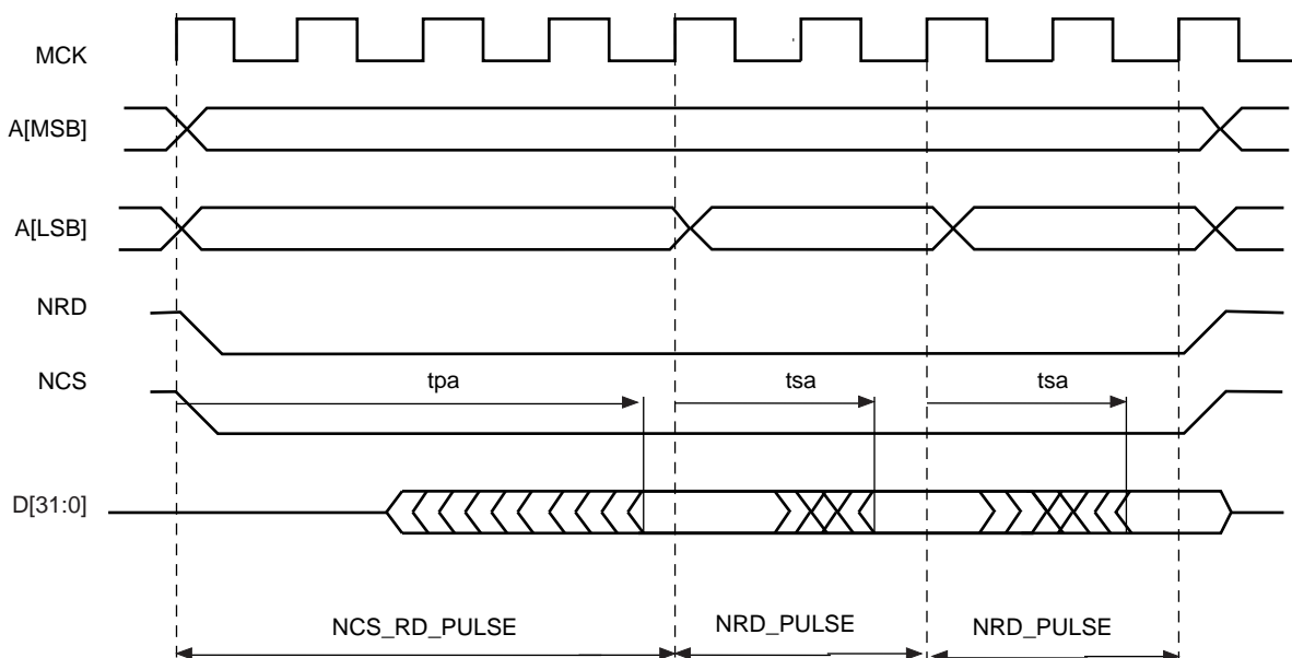
Figure 23-34. Page Mode Read Protocol (Address MSB and LSB are defined in Table 23-6 )
