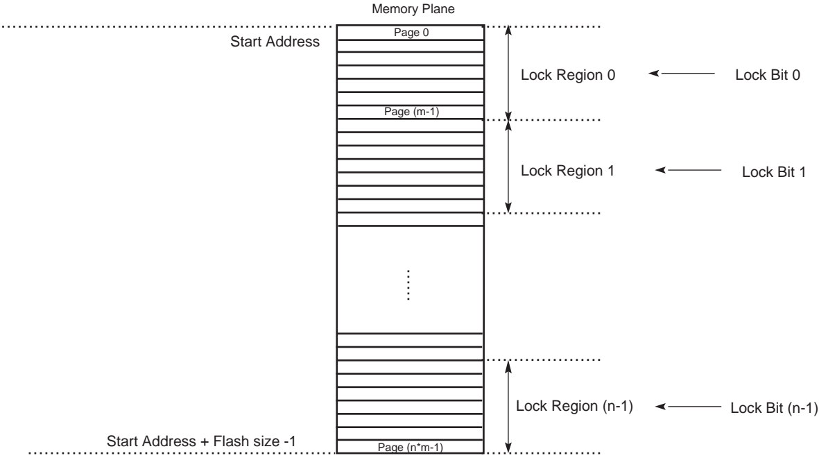
Figure 20-1. Embedded Flash Organization
