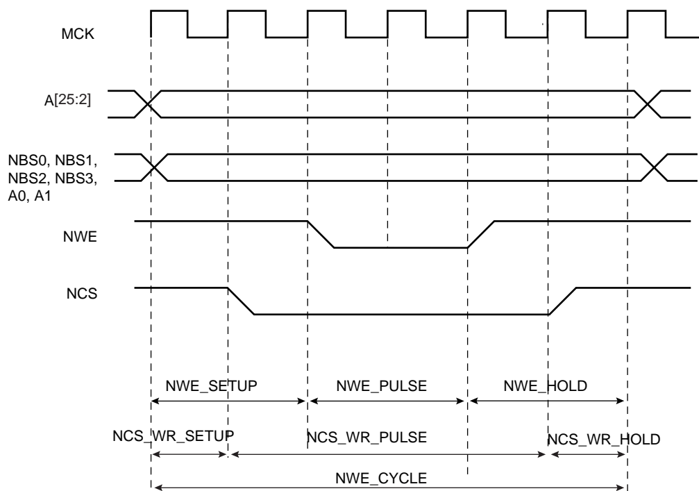
Figure 23-12. Write Cycle
