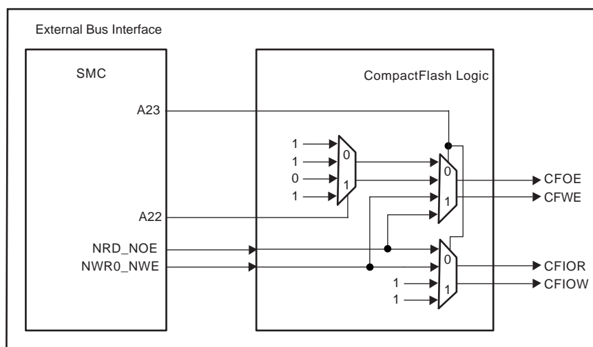
Figure 22-4. CompactFlash Read/Write Control Signals
