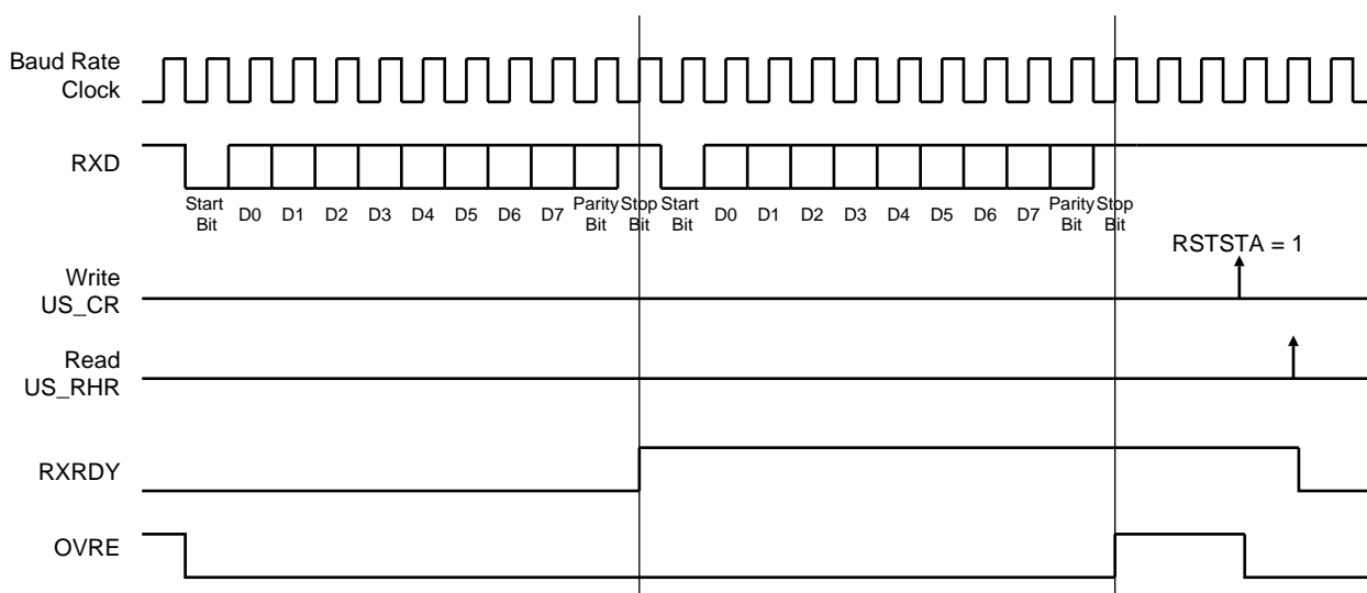
Figure 34-21. Receiver Status
