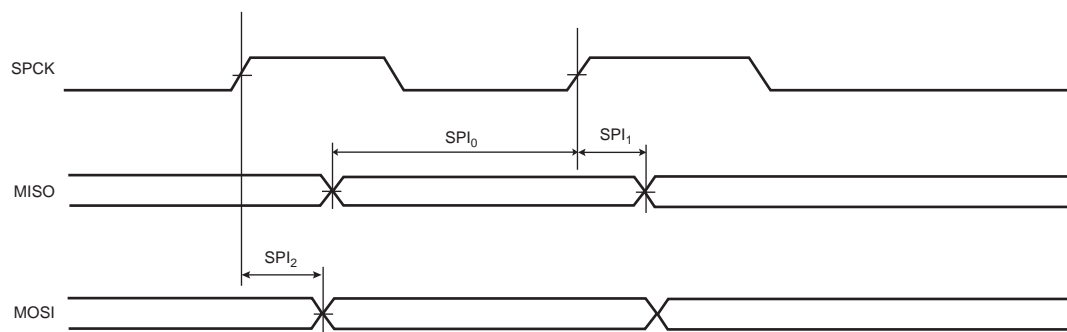
Figure 43-6. SPI Master Mode 1 and 2
