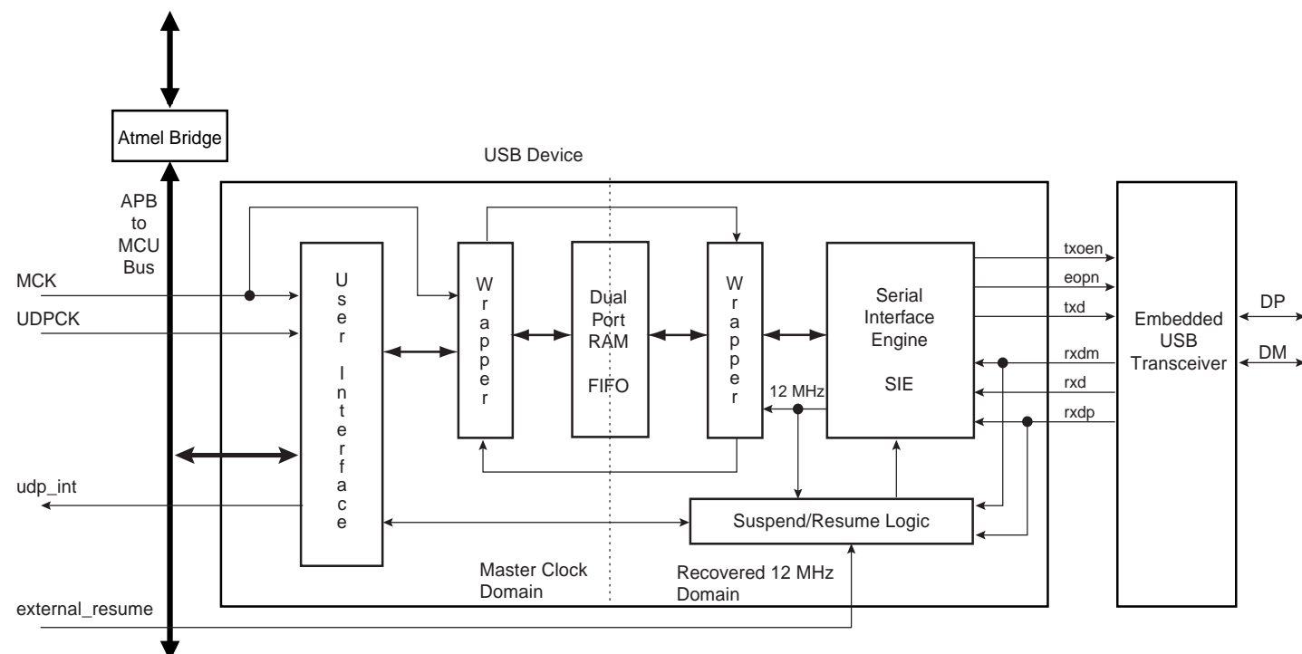
Figure 39-1. Block Diagram
