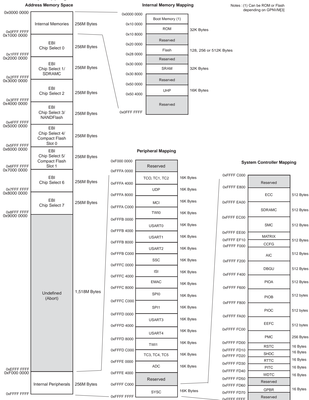
Figure 8-1. Memory Mapping
