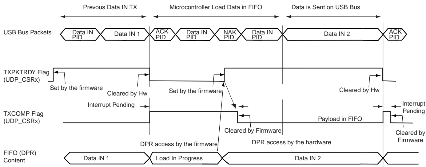
Figure 39-6. Data IN Transfer for Non Ping-pong Endpoint
