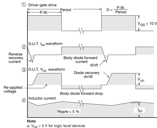
Fig. 20 - For N-Channel
