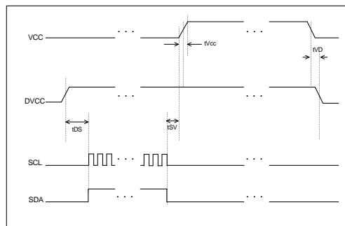
Power supply sequence diagram
